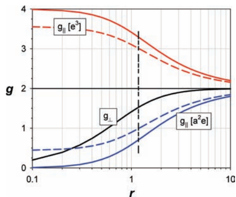
Figure 3. Plot of g -values for the [2e^3] and [3a_1^2 2e^1] configurations as a function of r (eq 10). The solid red and blue lines represent the crystal field limit, k = 1 ; the dashed lines include d-electron delocalization of (1 - k) = 22\% ; the vertical black dashed line indicates the r -value corresponding to the observed g -values of [\text{Mo}]N_2 and [\text{Mo}]CO in toluene.
