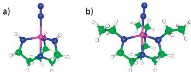
Figure 6. Ball-and-stick visualization of [\text{Mo}]_{\text{N}_2} model geometries \mathbf{1}' (a) and \mathbf{1}'' (b). The HIPT groups have been replaced by hydrogen atoms (a) or ethyl groups (b). Model \mathbf{1}' geometries were optimized on a CASSCF(3,2)/TZVP/ZORA level of theory. Model \mathbf{1}'' originates from optimizations of the full geometry including HIPT groups on a BP86/TZVP(Mo,N)/SV(P)(C,H)/ZORA level of theory. The subsequently introduced ethyl groups were optimized separately with the same method.
