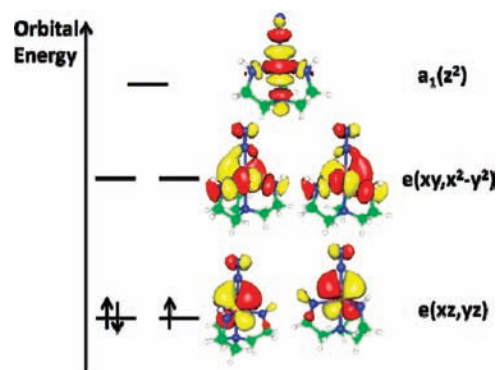
Figure 7. Qualitative molecular orbital diagram for the electronic ground state of \mathbf{1}' as obtained from MR-DDCI2: CAS(3,5)/TZVP/ZORA calculations. Shown are natural orbitals.
